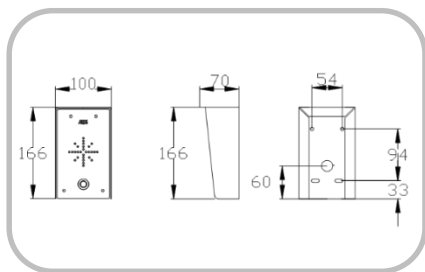
▶ 603-IMP CALL PANEL
