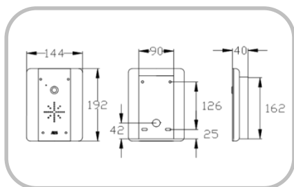
▶ 603-AB/AS CALL PANEL
