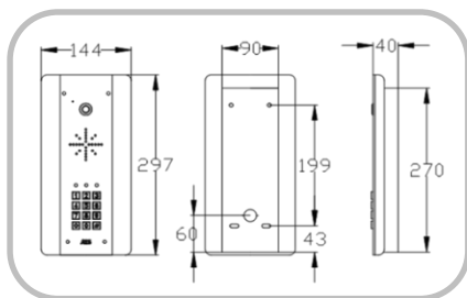
▶ 603-ABK/ASK CALL PANEL
