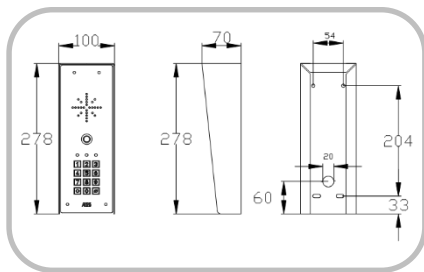
▶ 603-IMPK CALL PANEL
