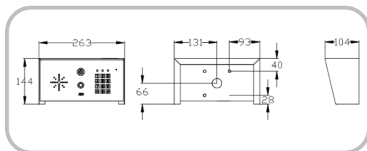
▶ 603-IMPK-PED CALL PANEL
