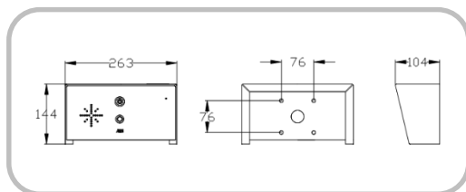
▶ 603-IMP-PED CALL PANEL
